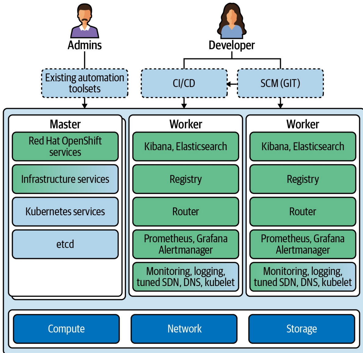
Figure 5-8. A simplified view of the OpenShift Container Platform stack and an abstraction of Kubernetes at the core of the platform
