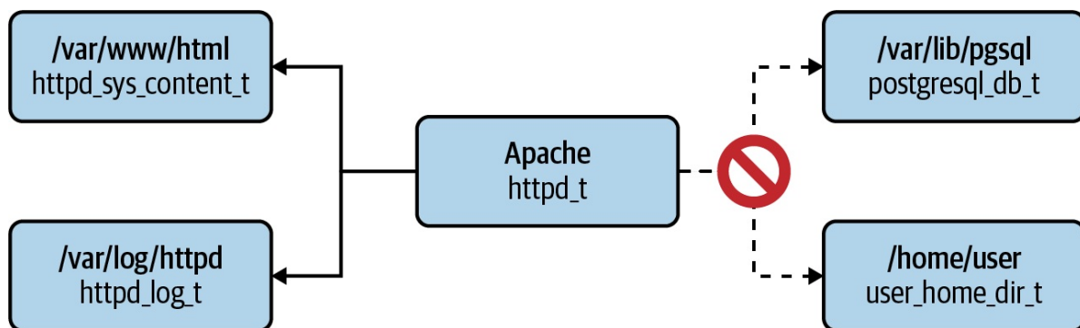
Figure 5-7. A depiction of SELinux “context” at work in securing an Apache HTTP server application with regard to permitted access routes (the /var/ directories on the left) and disallowed routes (Apache cannot access the PostgreSQL database on the right): context is set on every object across the system
