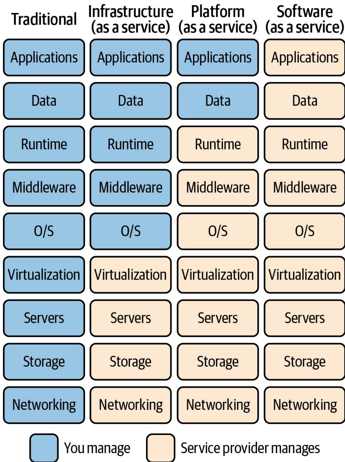
Figure 4-1. A high-level comparison of responsibilities at each cloud pattern level
